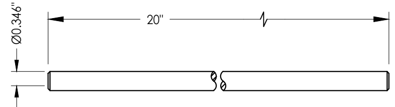
SLIDE BOLT ROD STEEL
